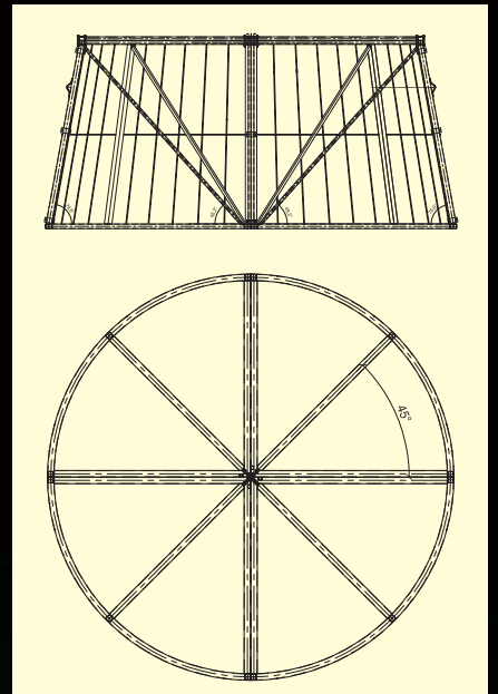
Cone's segment 12-14 / segment stożka 12-14
