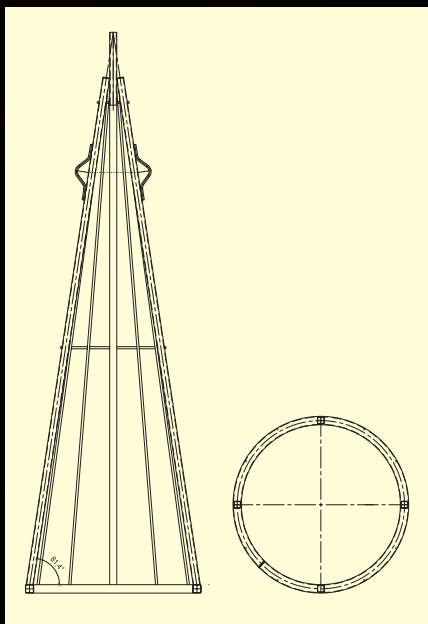
Cone's segment 0-2 / segment stożka 0-2
