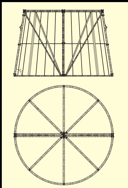
Cone's segment 8-10 / segment stożka 8-10
