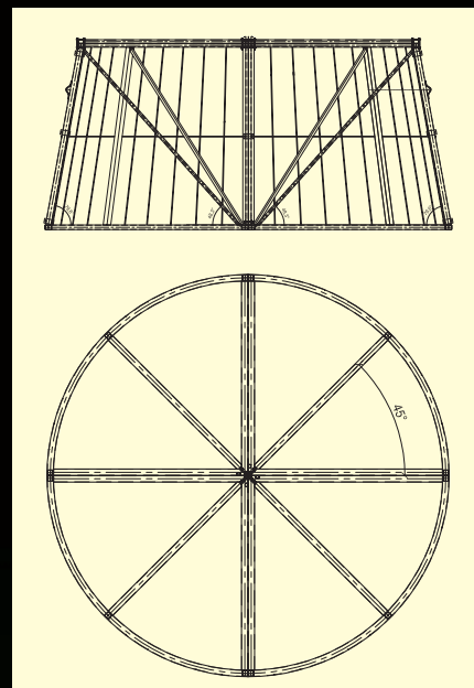
Cone's segment 12-14 / segment stożka 12-14
